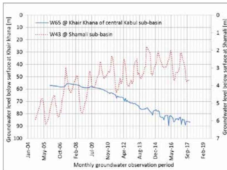
Figure 1.1: Example of extreme groundwater drawdown in Khair Khana area located at edges of central Kabul sub-basin (blue in left axis) and groundwater level rise as a result of groundwater regeneration in Shamali sub-basin (red, right axis)
